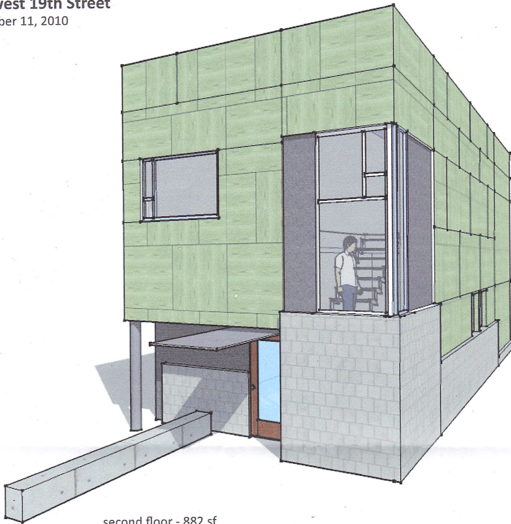
second floor - 882 sf
